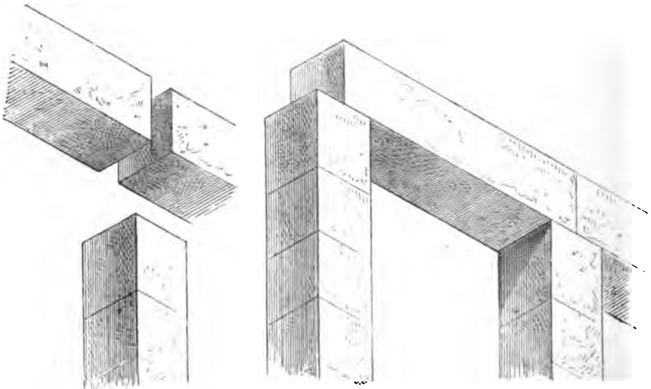
FIGS. 71, 72.—Elements of the portico.
